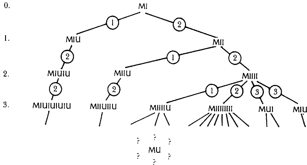
FIGURE 11. A systematically constructed “tree” of all the theorems of the MU-system. The Nth level down contains those theorems whose derivations contain exactly N steps. The encircled numbers tell which rule was employed. Is MU anywhere in this tree?
